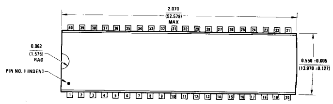
40-Lead Ceramic Dual-in-Line Package (D) Order Number INS8154D
