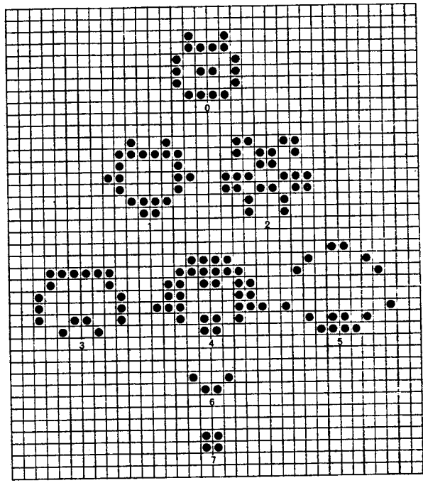
The Cheshire cat (0) fades to a grin (6) and disappears, leaving a pac print (7)
